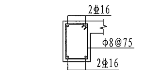
TL1 250 × 300
